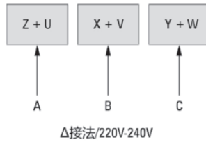
三相电机与刹车器接线方式 THE CONNECTION MODE FOR THREE PHASE MOTOR AND BRAKE
