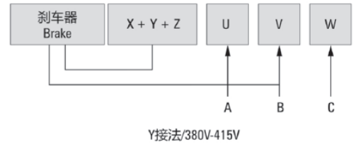
三相电机与刹车器接线方式 THE CONNECTION MODE FOR THREE PHASE MOTOR AND BRAKE
