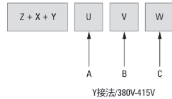
三相电机与刹车器接线方式 THE CONNECTION MODE FOR THREE PHASE MOTOR AND BRAKE
