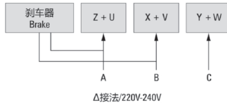
三相电机与刹车器接线方式 THE CONNECTION MODE FOR THREE PHASE MOTOR AND BRAKE
